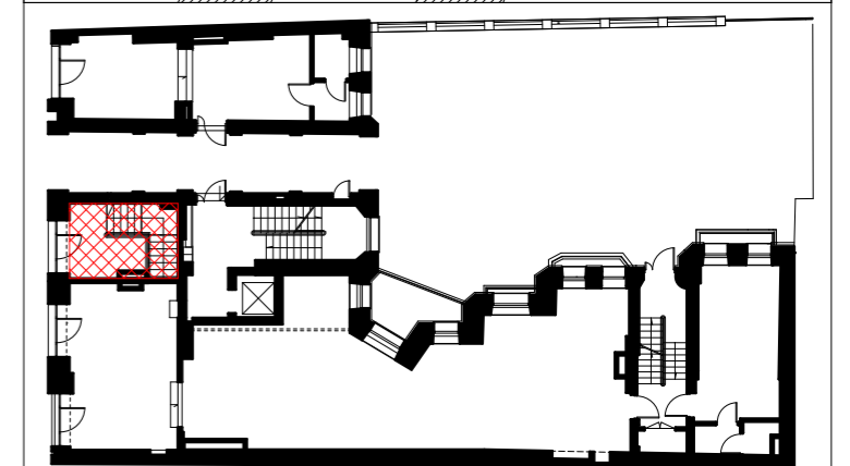
SCHEMAT PARTERU
